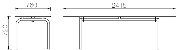
#2415.2 PB_CR Chrome/Glass
